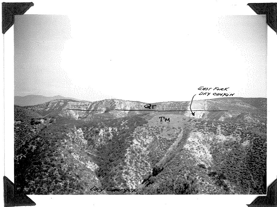
Fig.16 Terrace deposits.
